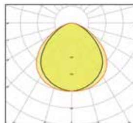
BEAM ANGLE
