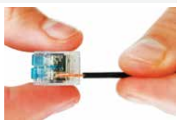
Fio descarnado até 10mm Strip conductor to 10mm Cable conductor de hasta 10mm
